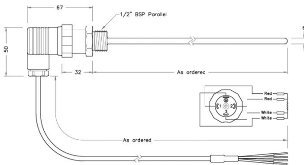
'HIRSCHMANN PT100 PROBE ASSEMBLY'
