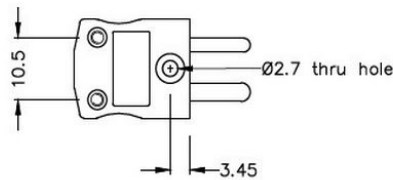
Miniature in-line Plug (dimensions in mm)
