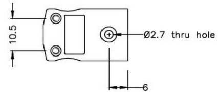
Miniature in-line Socket (dimensions in mm)
