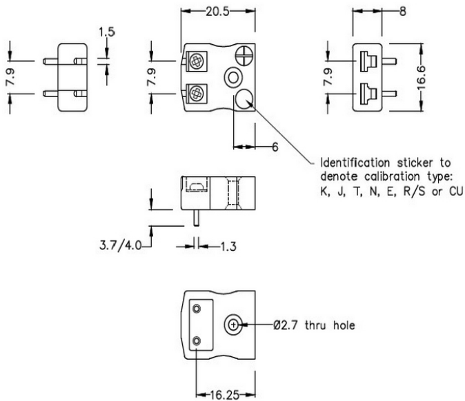
Miniature PCB Socket (dimensions in mm)
