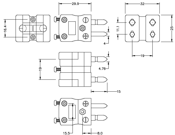
Standard Duplex in-line Plug (dimensions in mm)
