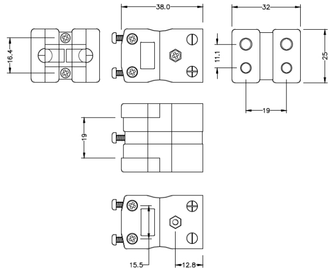
Standard Duplex in-line Socket (dimensions in mm)
