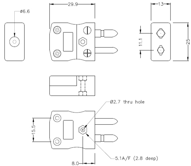
Standard in-line Plug (dimensions in mm)
