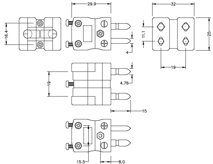
Standard Duplex in-line Plug (dimensions in mm)
